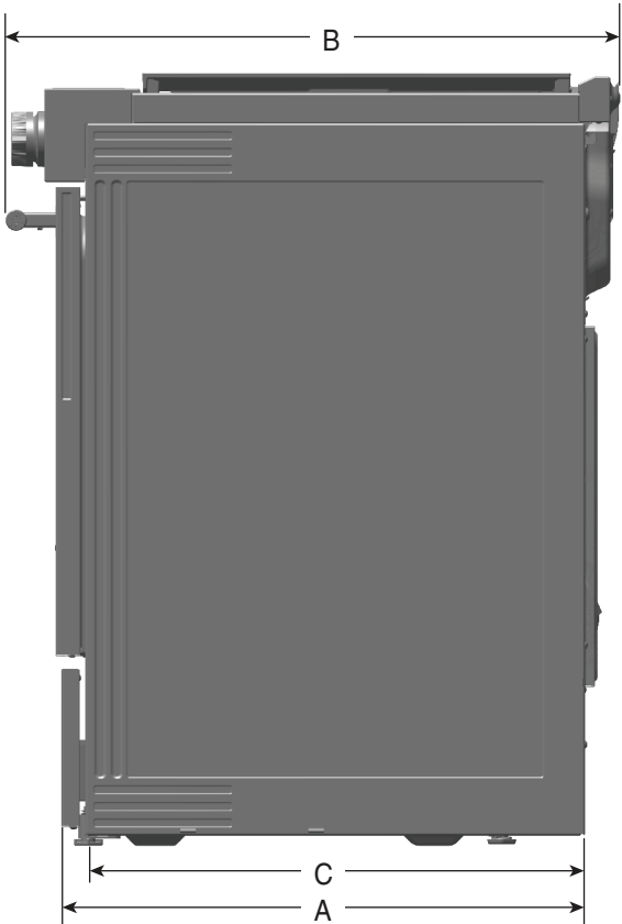
SIDE VIEW
