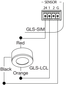
Switch Settings for Analog Input (Crestron Photocells, e.g., GLS-LCL and GLS-LOL)
