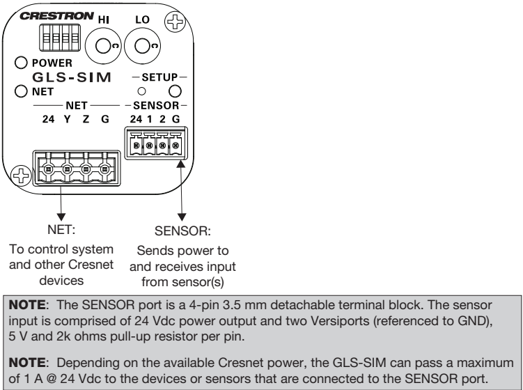
GLS-SIM Connections
