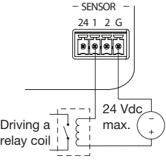
Switch Settings for Digital Output (Drive a Relay Coil)
