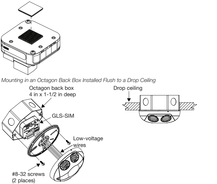
Using a Dual-Lock Fastener on the GLS-SIM (Optional)
