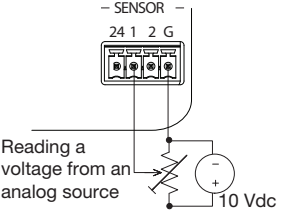
Switch Settings for Analog Input (Read Voltage from Analog Source)
