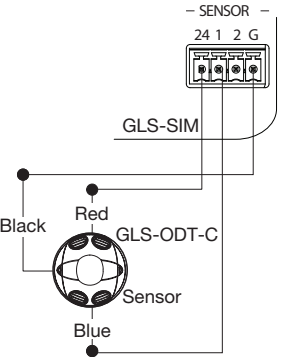
Switch Settings for Digital Input (Crestron occupancy sensors, e.g., GLS-ODT-C500/1000/2000)
