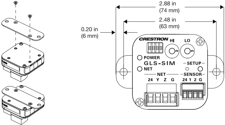
Attaching the Mounting Bracket to GLS-SIM (Optional)
