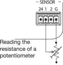
Switch Settings for Analog Input (Read Resistance of Potentiometer)
