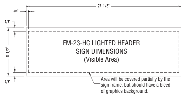
HEADER DIMS
