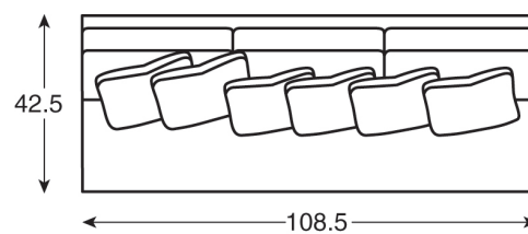
LTD5220-92 | Armless Sofa w 108.5 d 42.5 h 36 inside: w 108.5 d 22 h 16.5 seat: 19.5 6 std throw pillows: (3) 24 x 24 (3) 22 x 22
