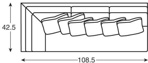
LTD5220-42 | LAF Sofa w 108.5 d 42.5 h 36 inside: w 93 d 22 h 16.5 seat: 19.5 arm: 36 6 std throw pillows: (1) 26 x 26 (1) 24 x 24 (4) 22 x 22
