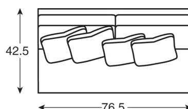
LTD5220-82 | Armless Love Seat w 76.5 d 42.5 h 36 inside: w 76.5 d 22 h 16.5 seat: 19.5 4 std throw pillows: (2) 24 x 24 (2) 22 x 22
