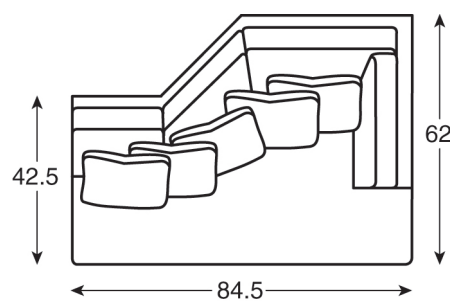
LTD5220-73 | RAF Drop Back Love Seat w 84.5 d 62 h 36 inside: w 69.5 d 33 h 16.5 seat: 19.5 arm: 36 5 std throw pillows: (1) 26 x 26 (1) 24 x 24 (3) 22 x 22
