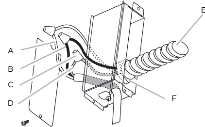
A. White wires B. Black wires C. UL listed wire connector D. Green (or bare) and yellow-green ground wire E. Home power supply cable F. UL listed or CSA approved 1/2" strain relief
