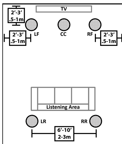
Figure 4.3: 5 Speaker Setup
