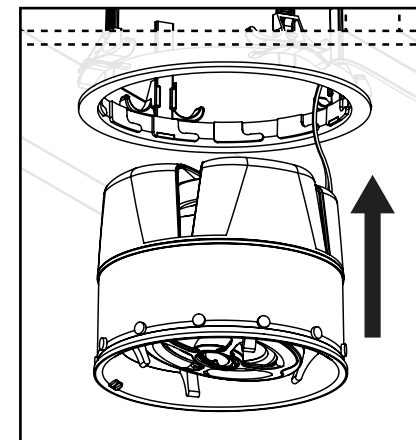
Figure 9.3: Insert Speaker
