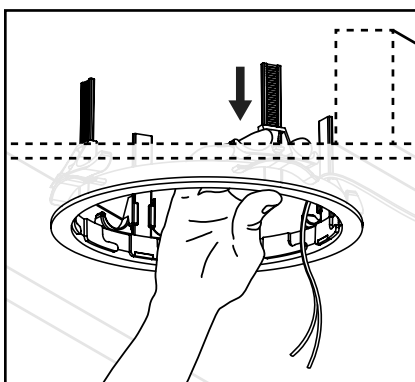
Figure 8.2: Lower ZipClip (2)
