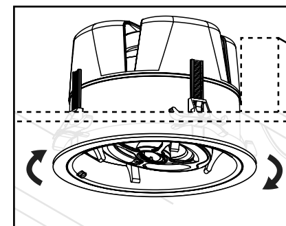
Figure 9.4: Secure Speaker
