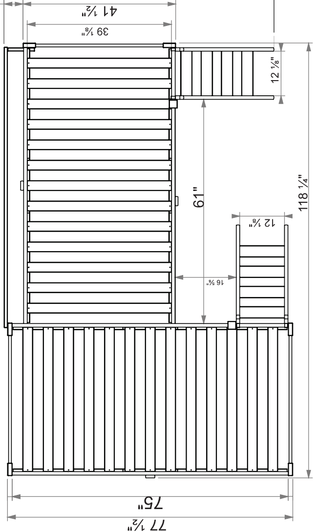
Top View
