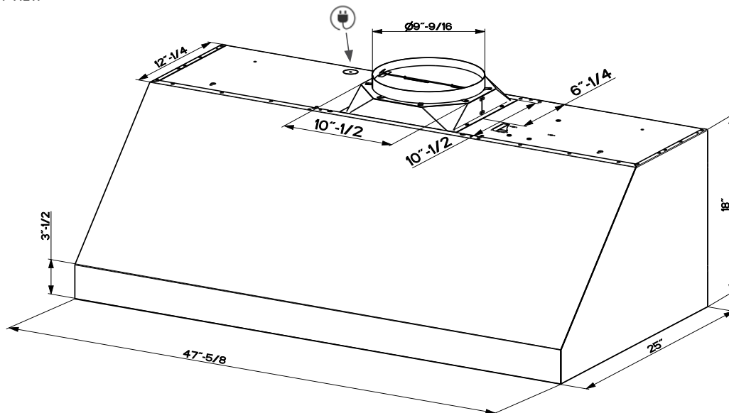
48" FRONT VIEW
