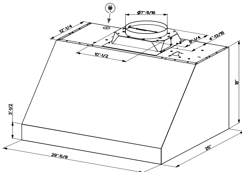
30° FRONT VIEW
