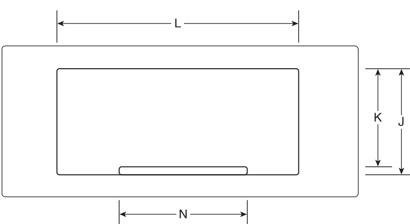
CAVITY INTERIOR FRONT VIEW
