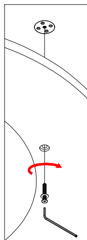
Detail 'C'
