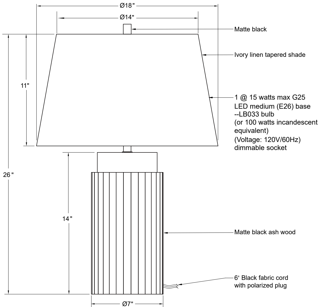
FRONT VIEW
