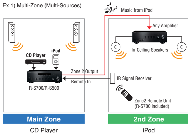
Ex.1) Multi-Zone (Multi-Sources)
