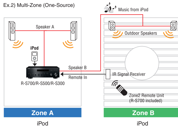
Ex.2) Multi-Zone (One-Source)
