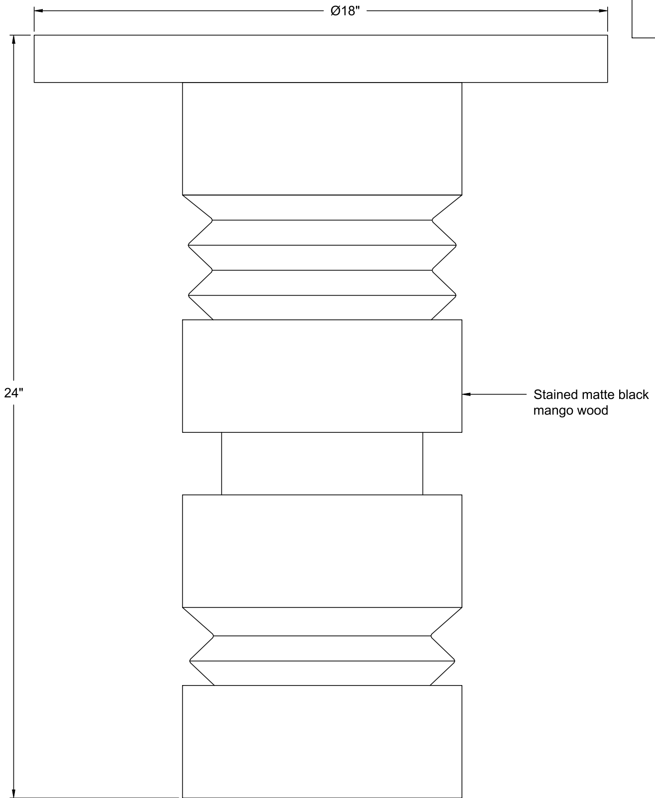
FRONT VIEW
