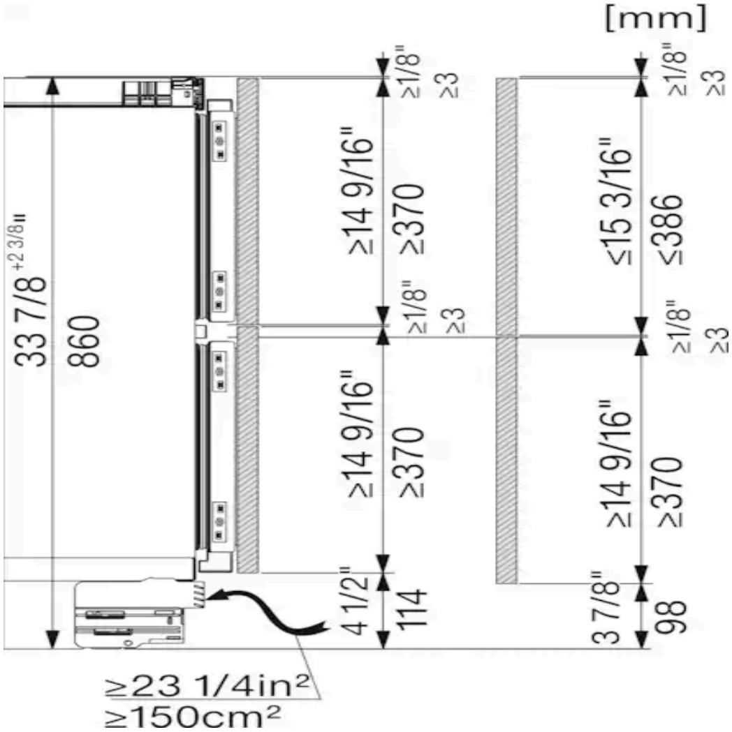
KU7175D, Built-under, side view
