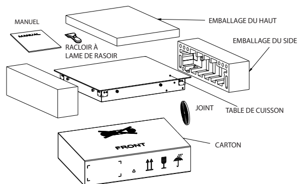
FIGURE 5 - PARTS
