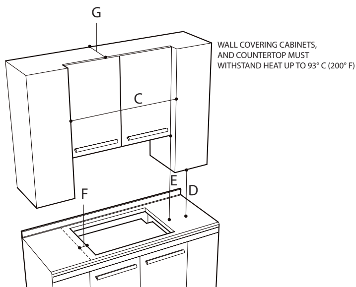
FIGURE 3 - CUTOUT REQUIREMENTS
