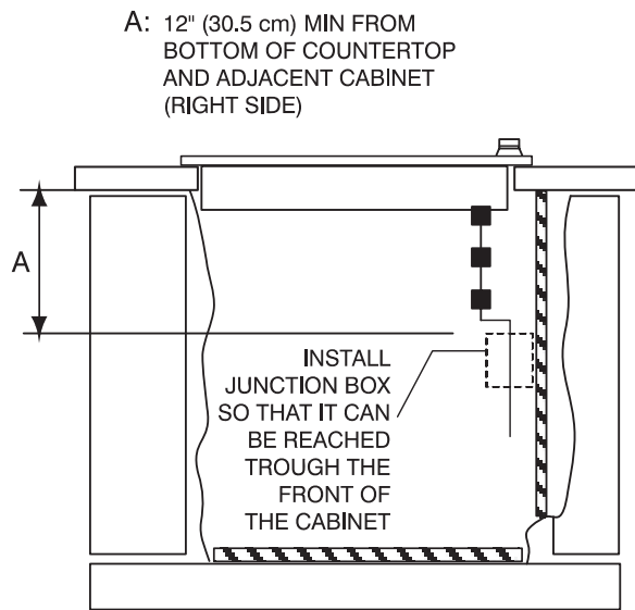
FIGURE 10 - ELECTRIC LINE OPENING
