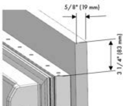
Assembly dimension between panel and refrigerator door
