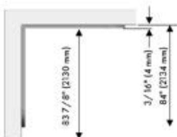
Anti-tip bracket location
