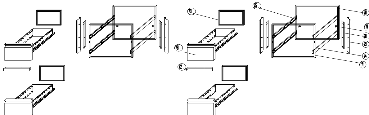
EXPLODE OF KCHMT60.24.4D
