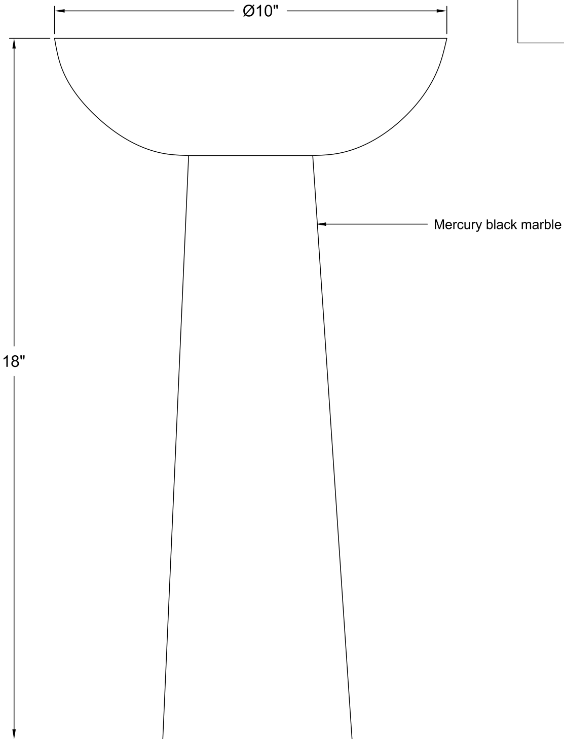
FRONT VIEW
