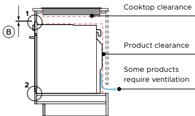
PROFILE VIEW
