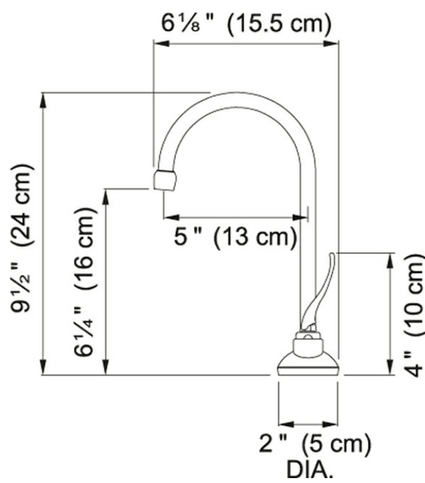
Technical Drawing
