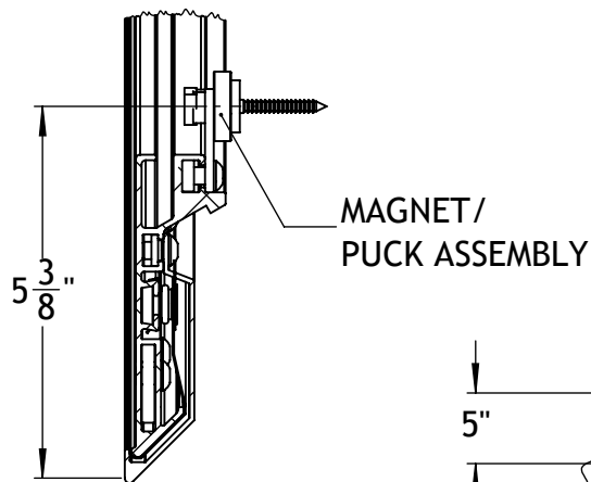
DETAIL C SCALE 1 : 3
