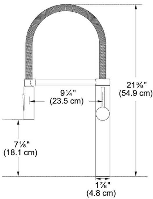
Technical Drawing
