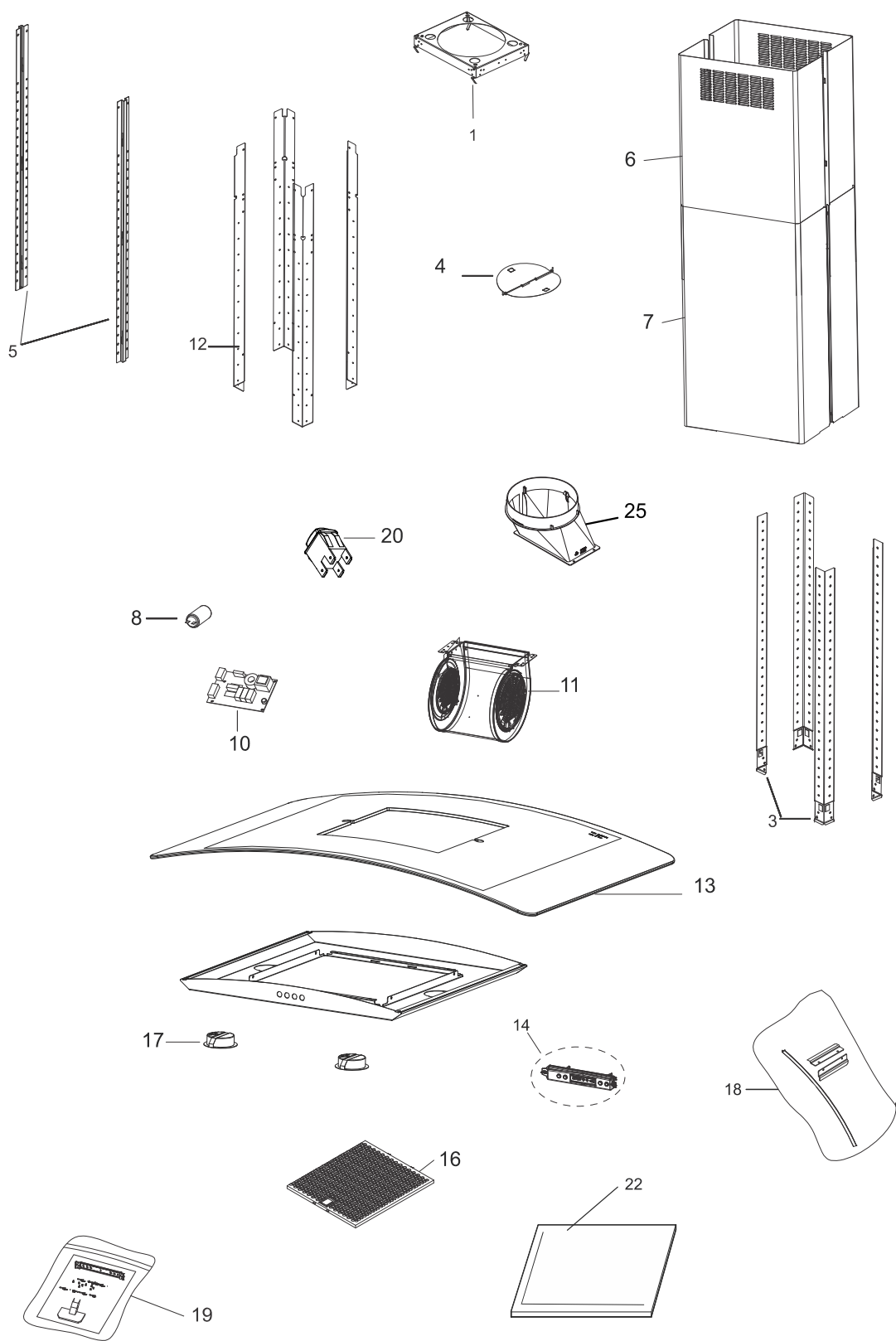
RH36PC60GSB1 Parts
