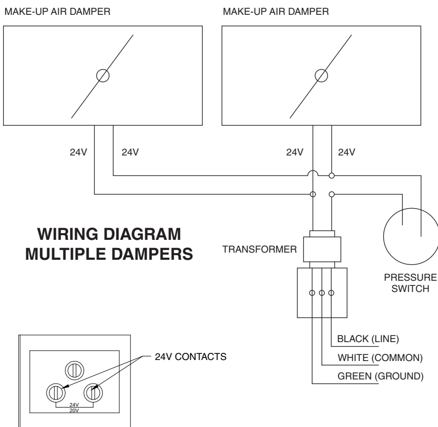
TRANSFORMER WIRING
