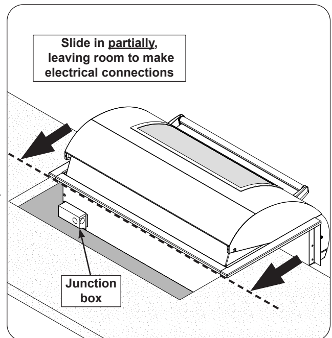
Fig. 26-2 Position unit for wiring
