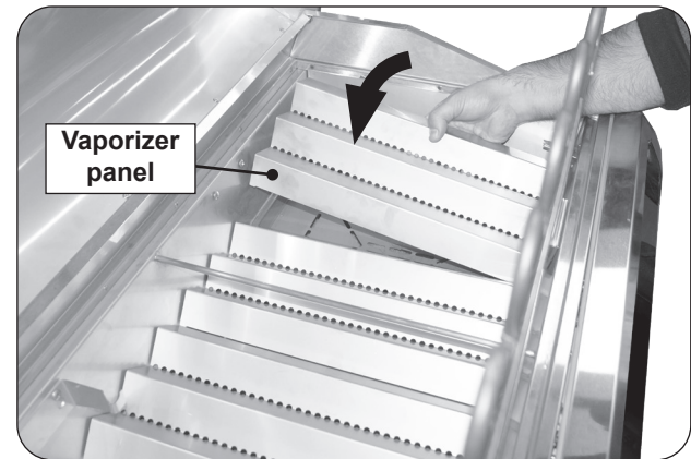
Fig. 28-2 Install vaporizer panels
