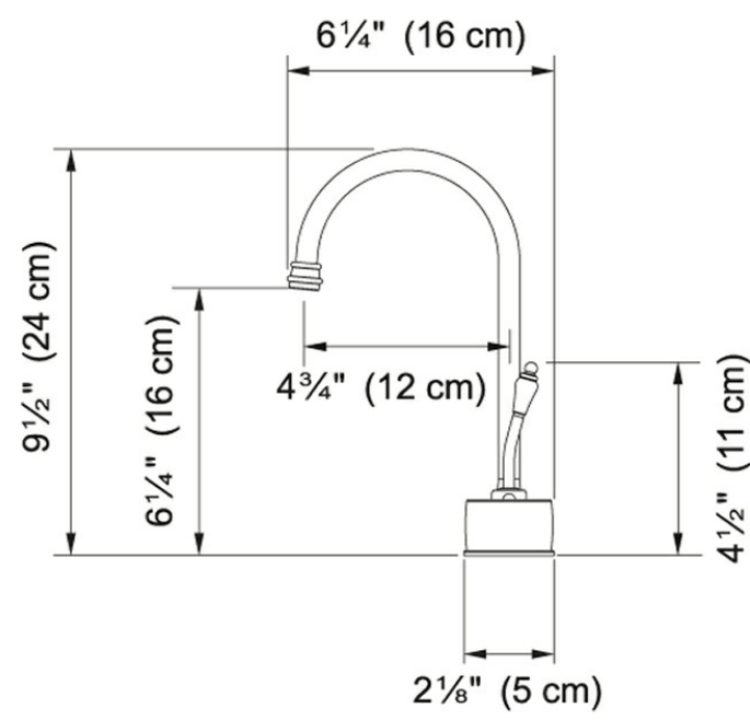
Technical Drawing
