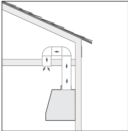
CEILING EXHAUST
