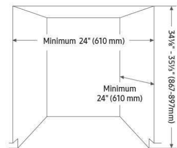
Cabinet size
