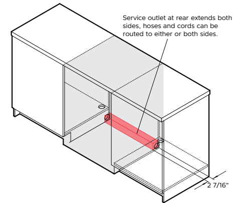
ISO VIEW
