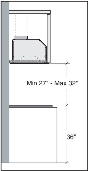
› Mounting height and clearance:
