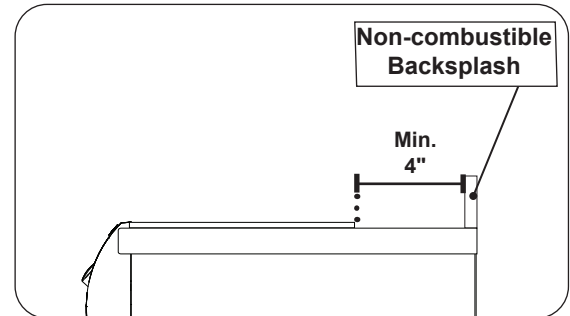
Fig. 18-4 Backsplash clearance
