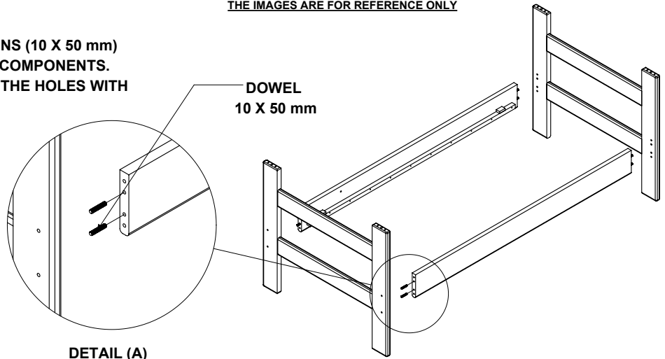
DETAIL (A)
