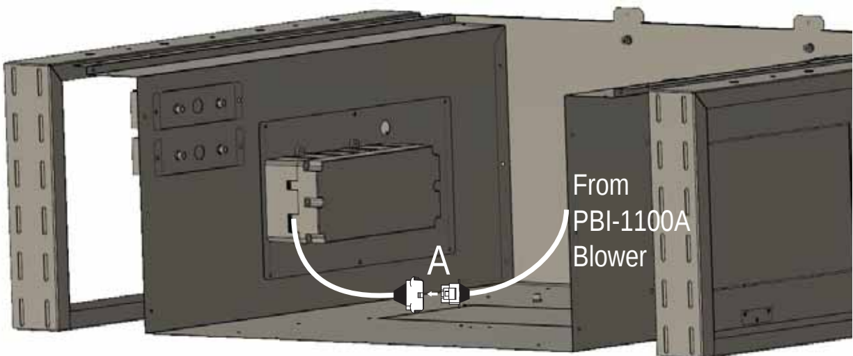
PBI-1100A Wiring
