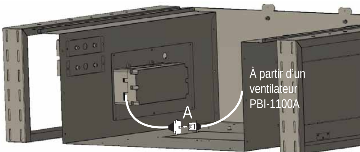
Câblage – PBI-1100A
