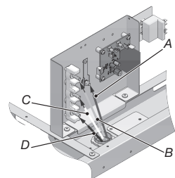
(type A vertical) 4-WIRE CONNECTION
