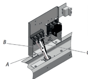
(type B) 3-WIRE CONNECTION
