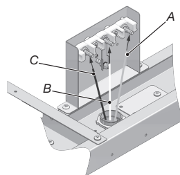
(type A orizontal) 3-WIRE CONNECTION
