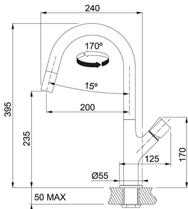
Technical Drawing
