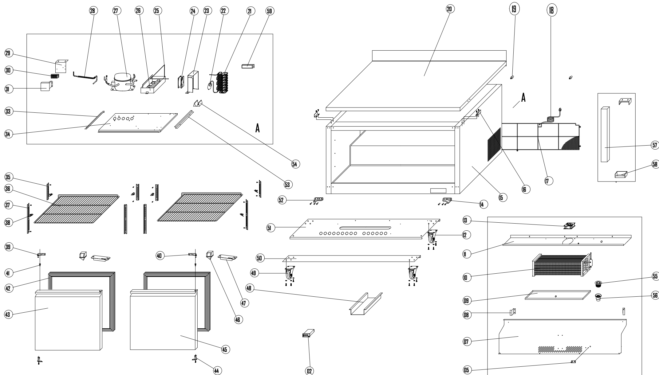
EXPLODE OF KCHUCWT60R
