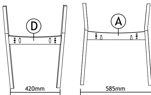
BACK LEG
