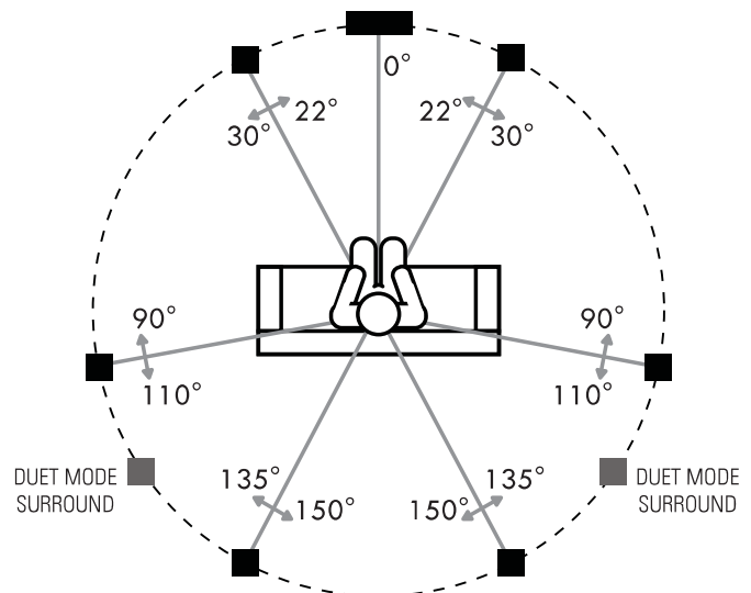
TYPICAL 7.0 SPEAKER PLACEMENT
