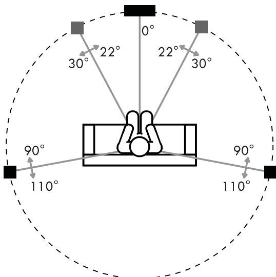
TYPICAL STEREO OR 5.0 SPEAKER PLACEMENT
