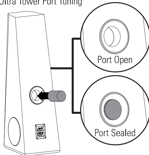
Ultra Tower Port Tuning
