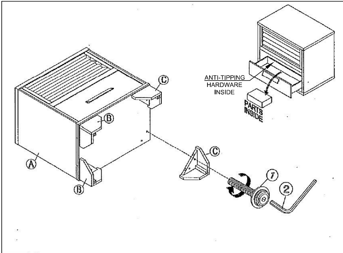
COMPLETED NIGHTSTAND ASSEMBLY
