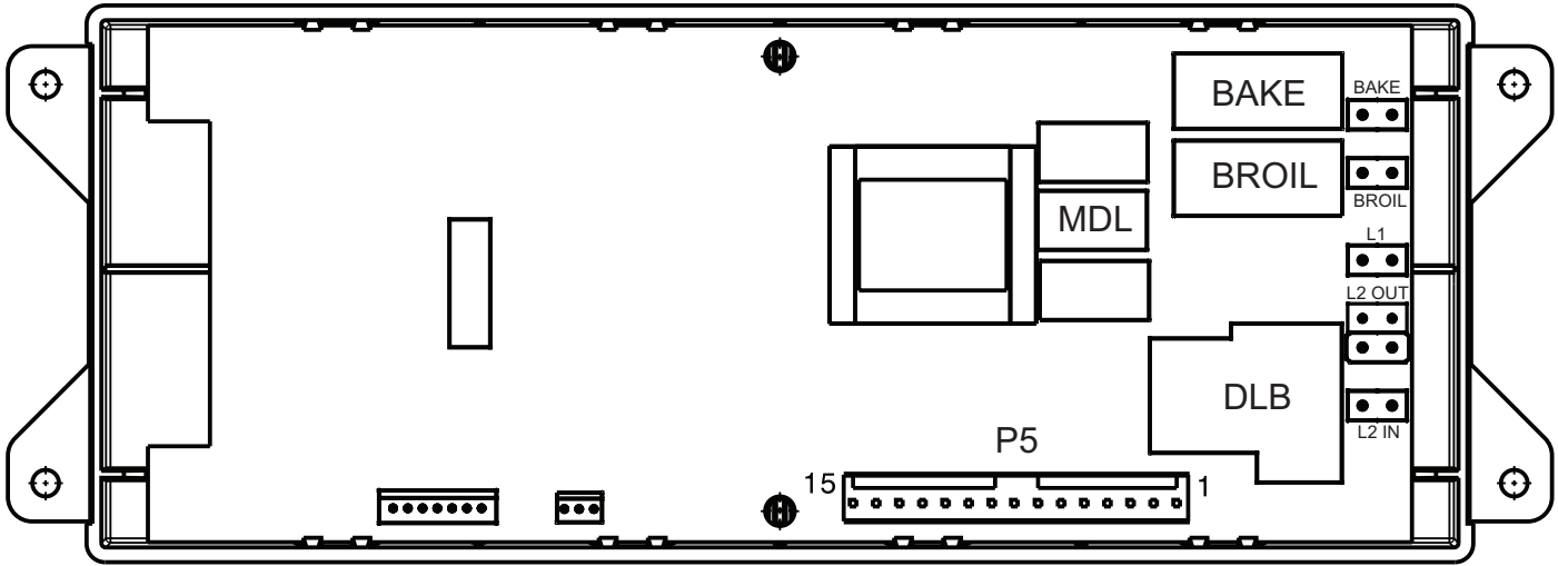
P5 CONNECTIONS
