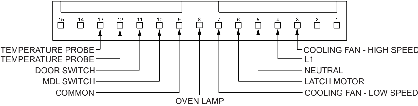
P5 CONNECTIONS
