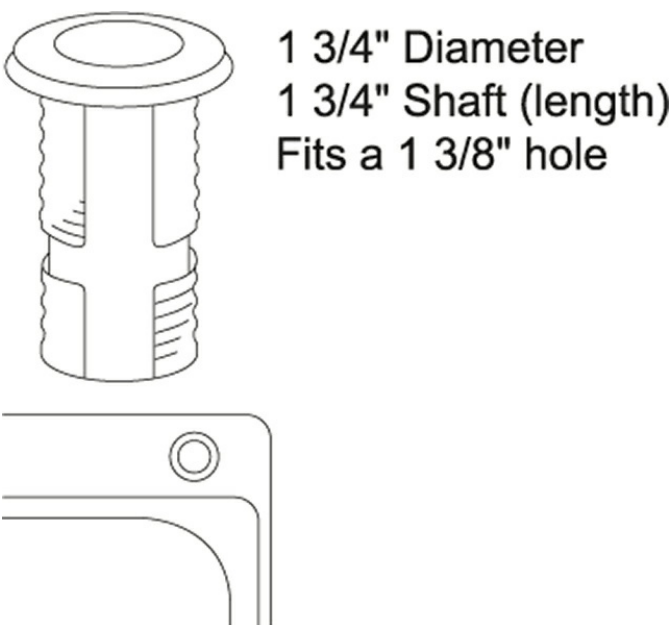
Technical Drawing
