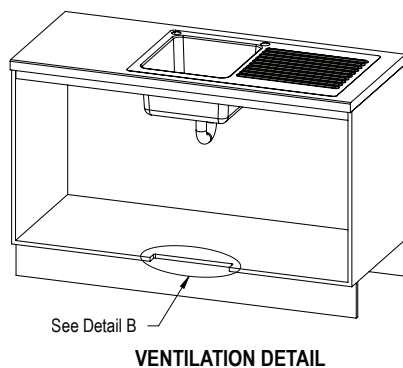
VENTILATION DETAIL
