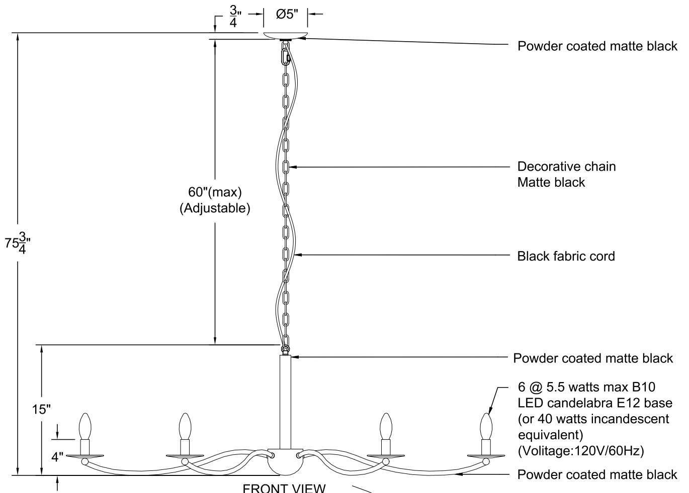
FRONT VIEW
