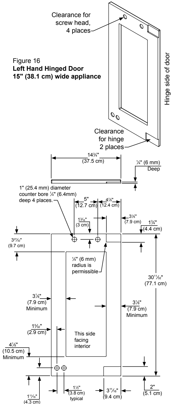
Figure 17 Left Hand Hinged Door 15" (38.1 cm) Wide Appliance
