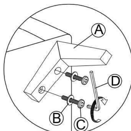
DETAIL 1.1
