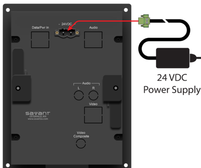
Rear View of OWC-200B
