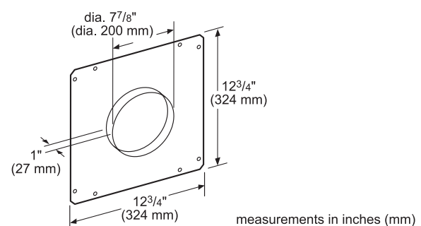
HDDFTRAN8 8" Round Front Plate for Downdraft
