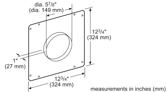
HDDFTRAN6 6" Round Front Plate for Downdraft
