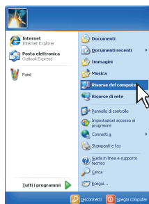
Windows XP
