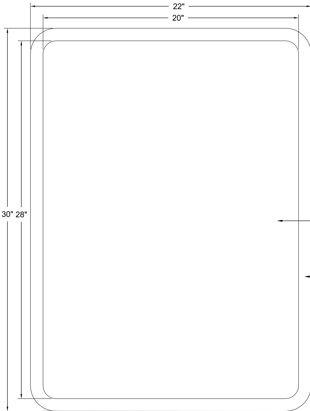
FRONT VIEW
