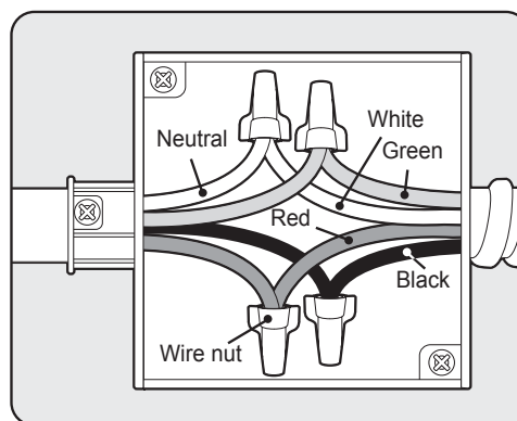
Junction Box
